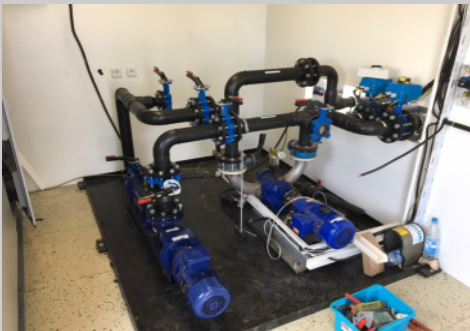
Pump system
