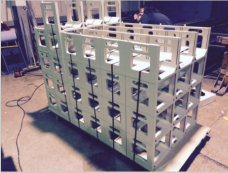
Milled parts
